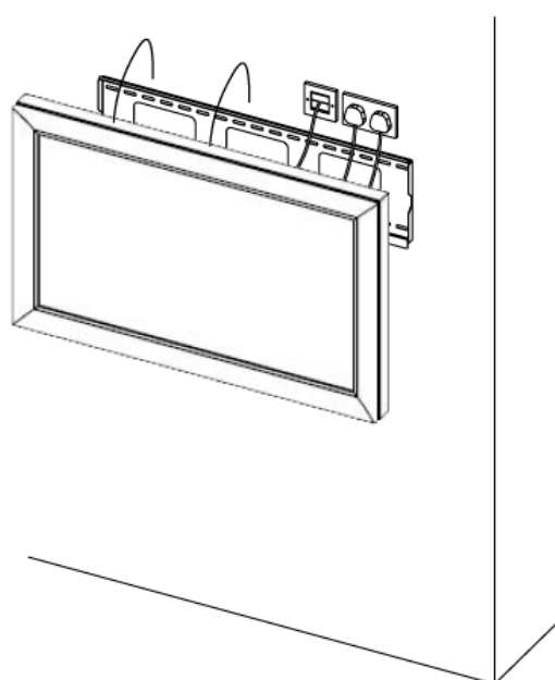
Step 2: Plug in TV and IR extender Mount the TV frame to the wall bracket.
